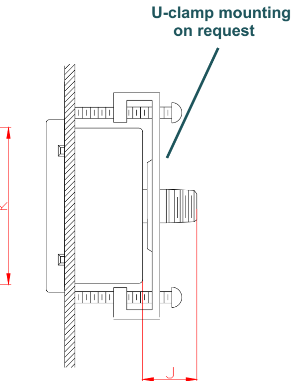
21B (Center Back Connection) Lower Back Connection on request
