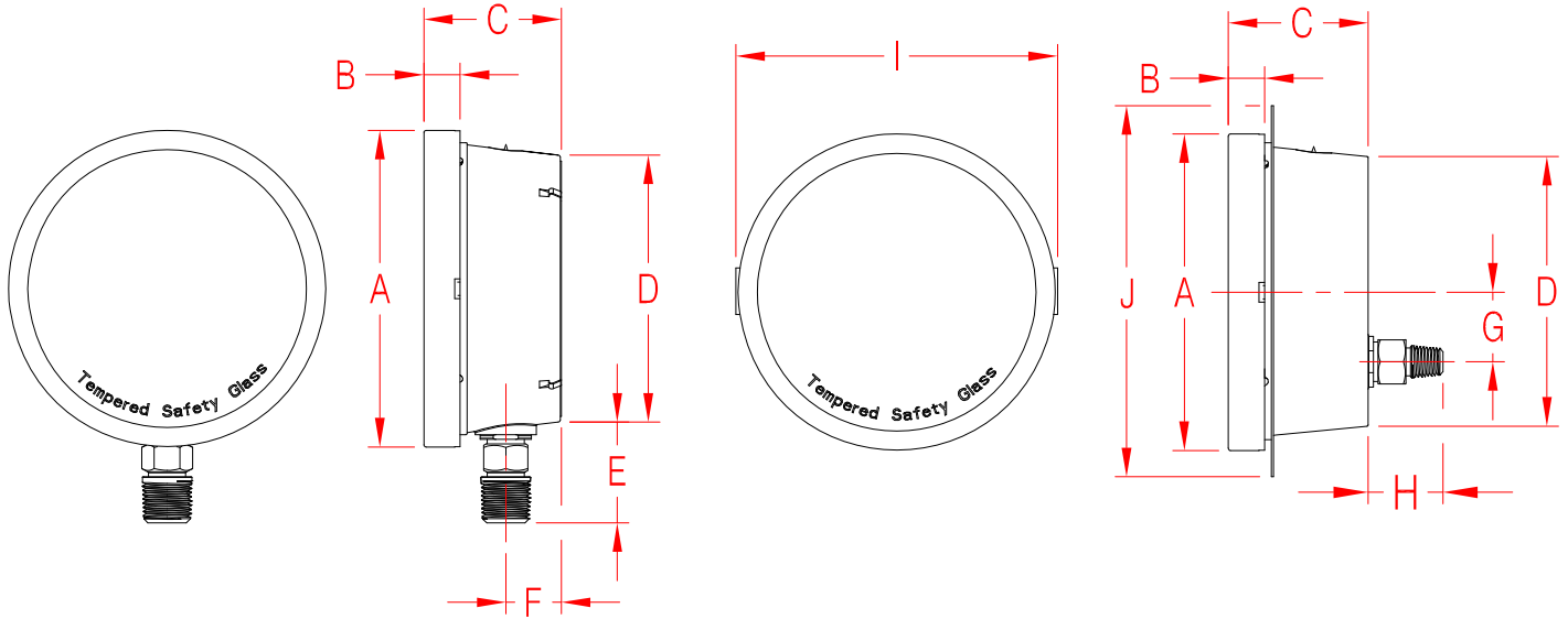
Bottom Connection
