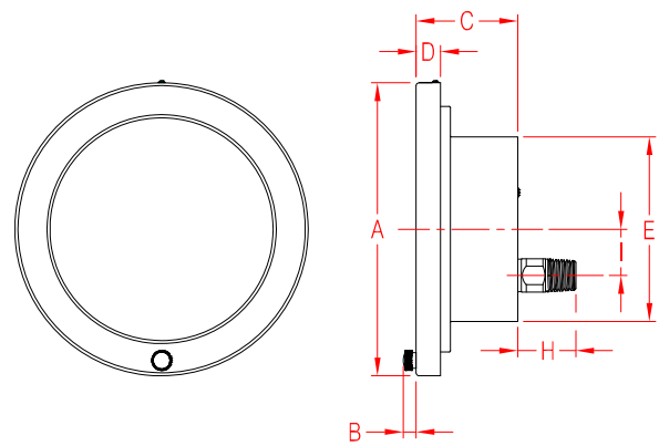
Back Connection
