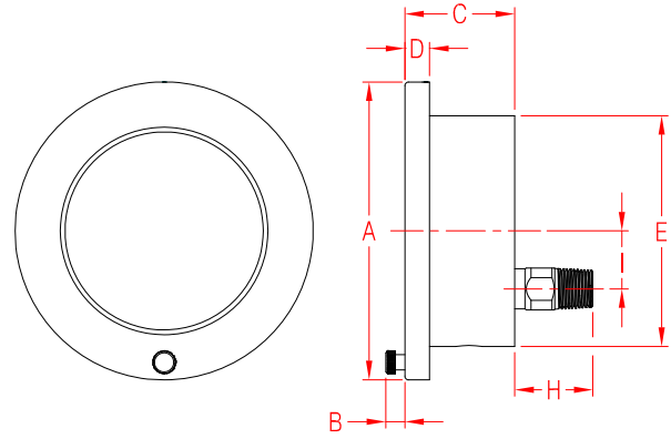
Back Connection
