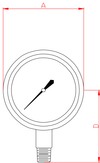
74L(Bottom Connection)
