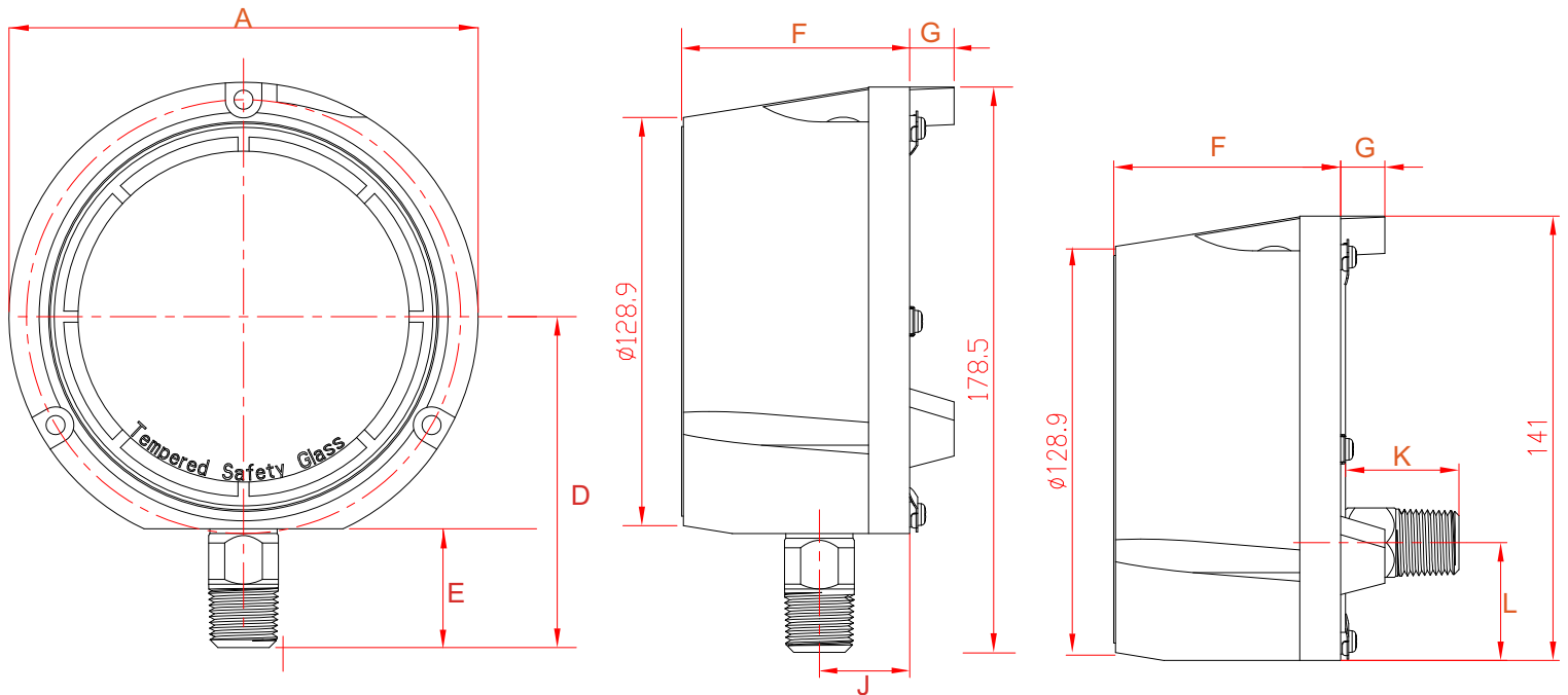
Dimensions, in.(mm)
